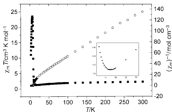
Fig. 8 \chi_m T (filled squares) and \chi_m^{-1} (open circles) versus temperature for compound I . The expanded view (inset) shows the minimum in \chi_m T .
